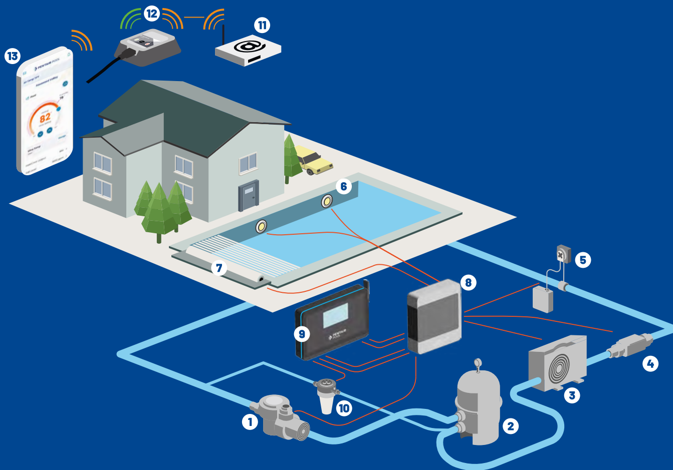
Example of a PoolGenius system installation
